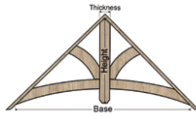
Arched Gable Bracket
