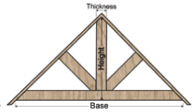
Straight Gable Bracket
